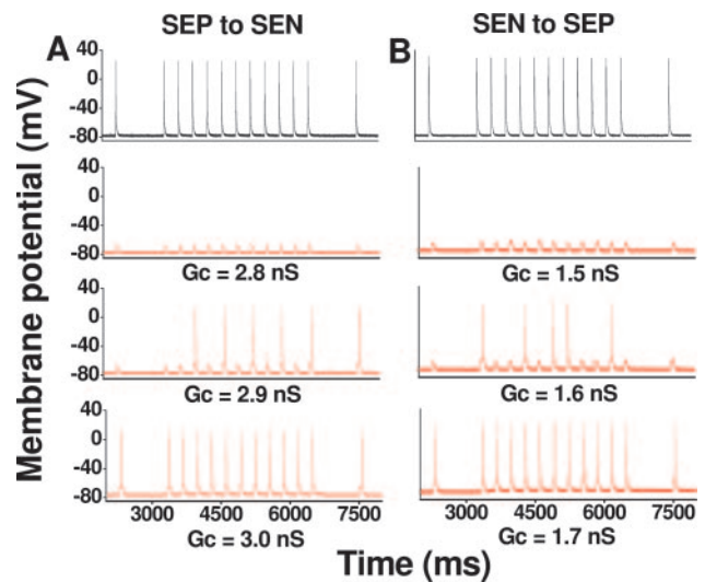
Figure 5. AP propagation in a coupled-cell pair from control mouse LV. Representative recordings from the leader cell are depicted in black, and recordings from the follower cell are in red. AP conduction from a subendocardial myocyte (SEN) to a subepicardial myocyte (SEP) (B) failed at G_c 1.5 nS. Increasing G_c to 1.6 nS led to partial impulse propagation. By further increasing G_c to 1.7 nS, all APs propagated successfully at both pacing frequencies (1 Hz, 3 Hz). For the same cell pair, however, AP propagation from SEP to SEN (A) required more coupling conductance: G_c 2.9 for partial propagation and G_c 3.0 for full AP propagation. Thus, there is unidirectional conduction block (from SEP to SEN) over a wide range of G_c (from 1.7 to 2.8).
