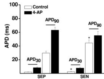
Figure 3. Changes in repolarization kinetics in mouse ventricular myocytes (n=10) in the absence and presence of 4-AP. Inhibition of I_{to} attenuates the transmural gradient of APD. APD 30 indicates APD at 30% repolarization; APD 90 , APD at 90% repolarization. * P < 0.05 compared with subepicardial myocytes (SEP). SEN indicates subendocardial myocytes.
