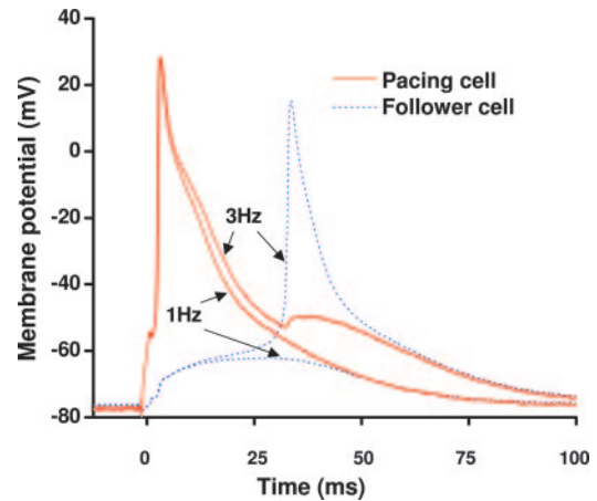
Figure 7. A replot of APs from Figure 6B (asterisks, third row) at a faster time scale. In failing myocytes, early repolarization of the AP is delayed immediately on increasing stimulation frequency, contributing to facilitated cell-cell electrotonic coupling.
