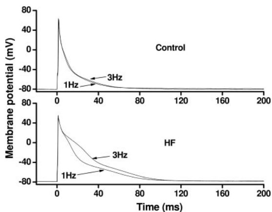
Figure 4. Frequency-dependent changes in AP profile differ between myocytes isolated from sham-operated control LV and from failing LV. Depicted here are representative, frequency-dependent AP waveform changes from 2 subendocardial myocytes.
