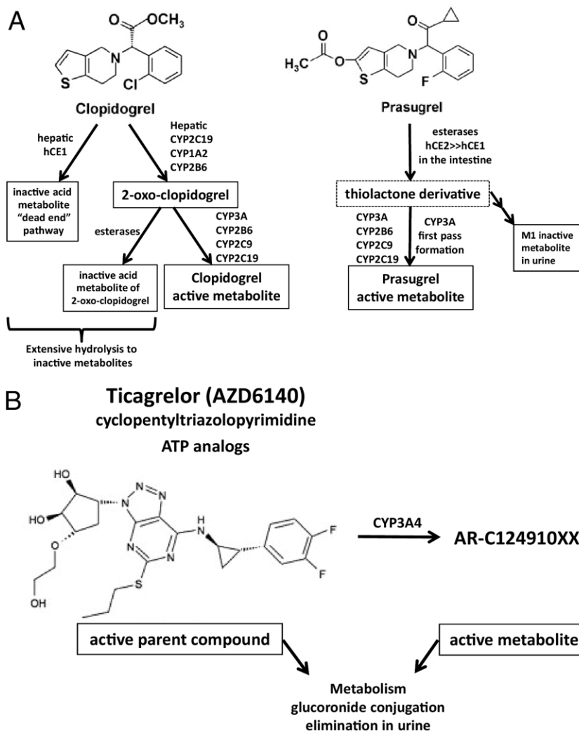
Figure 1. Thienopyridine Metabolism
